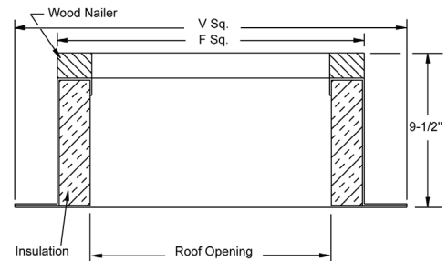
Pre-Fabricated Curb Dimension Data
