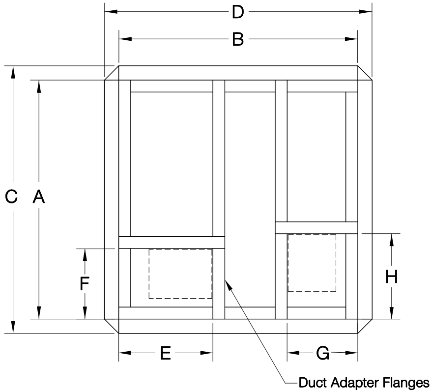
ERV CURB TOP VIEW ARR. V
