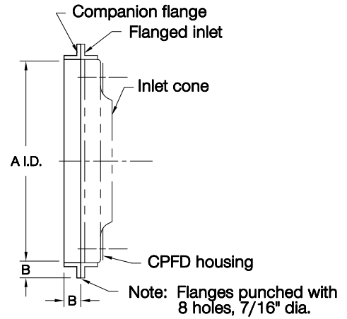
CPFD FLANGED INLET WITH COMPANION FLANGE
