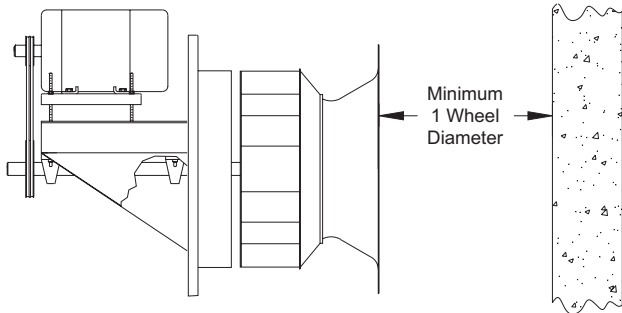
Figure 1 - Non-Ducted Inlet Clearance
