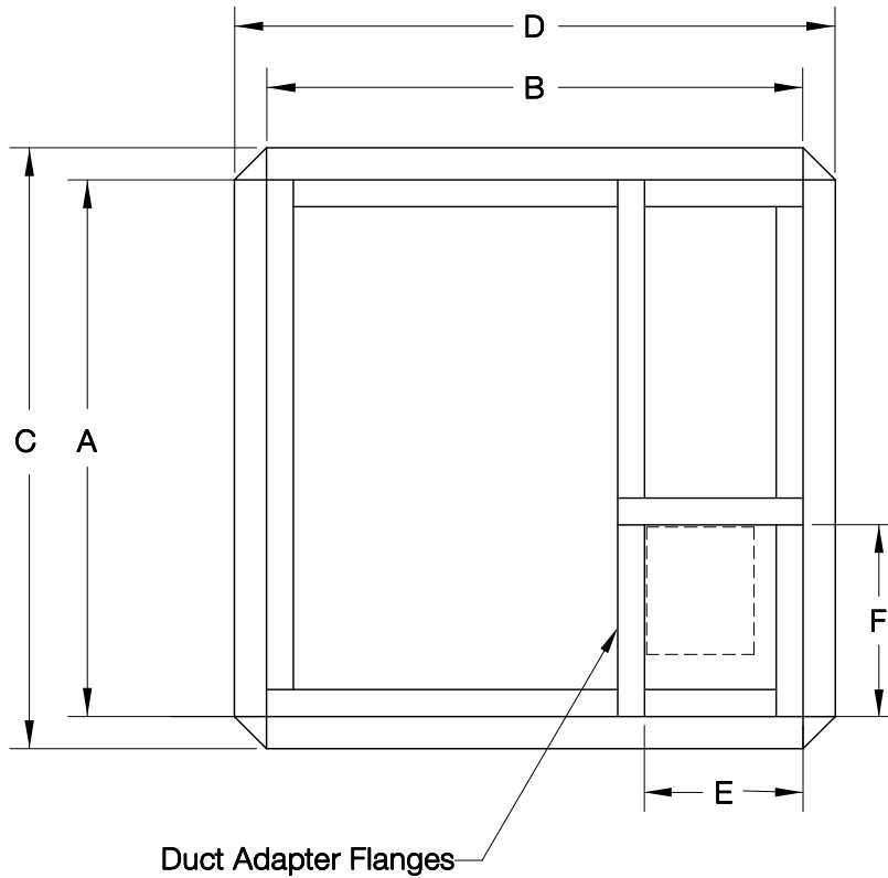
ERV CURB TOP VIEW ARR. C
